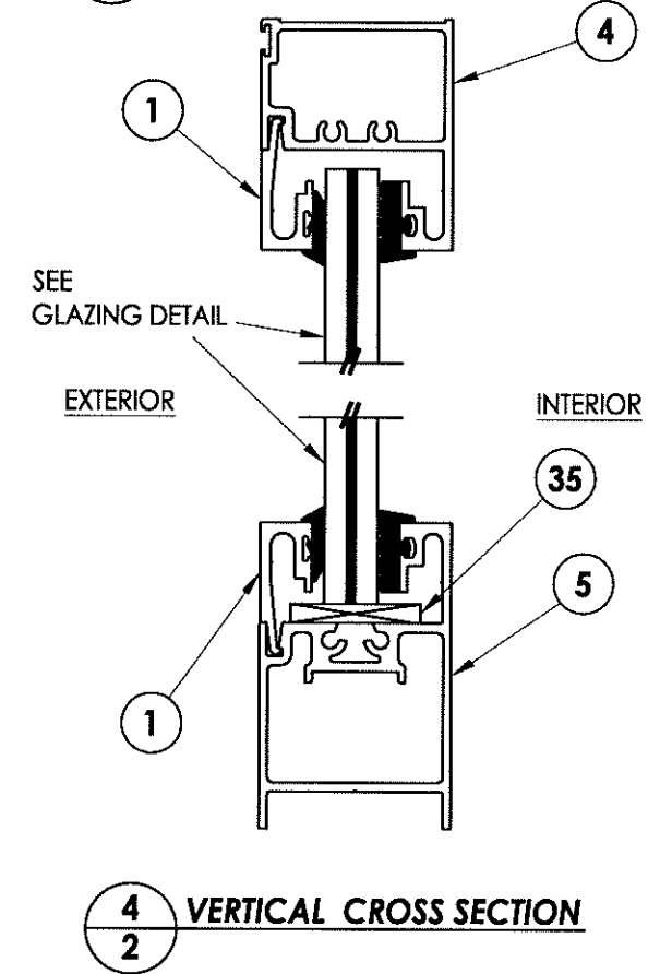
2/2 VERTICAL CROSS SECTION
