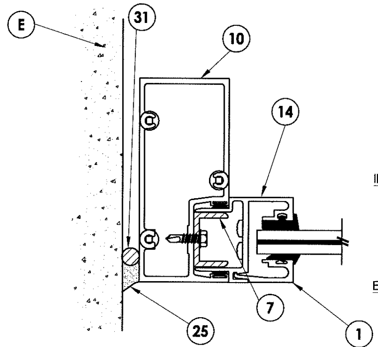
1 7 HORIZONTAL CROSS SECTION
