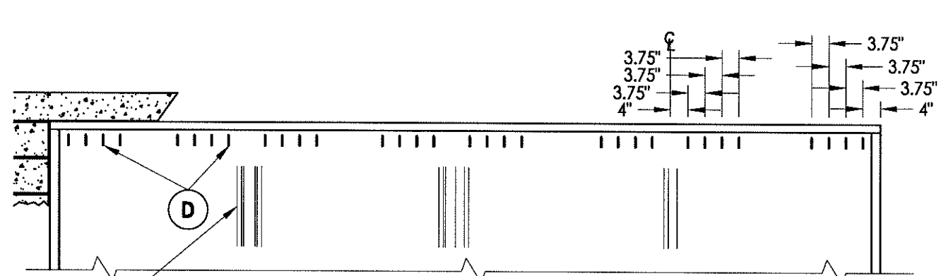
FRAME ANCHORING @ HEAD DP <= 135 PSF Max. shim space <= .25"
