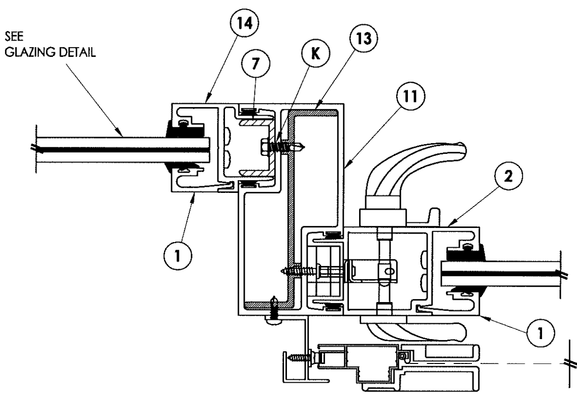
3 6 HORIZONTAL CROSS SECTION
