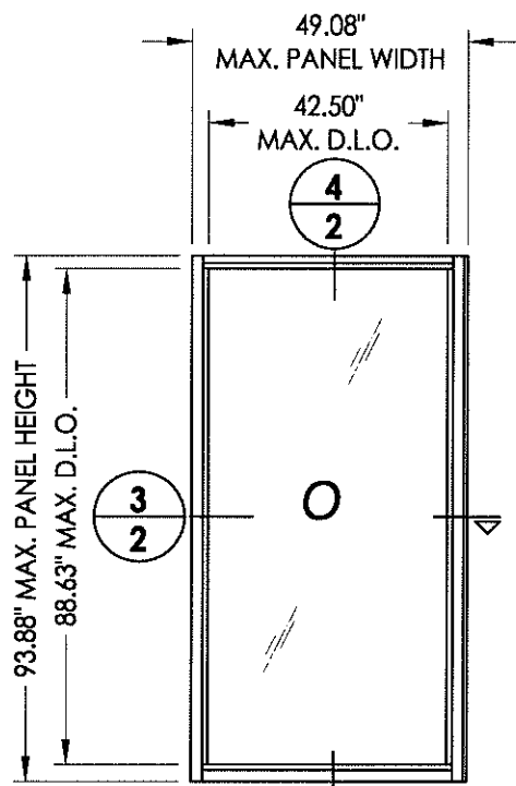
FIXED PANEL
